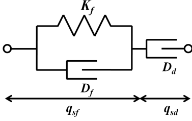
Fig. 1 Three-element model.
